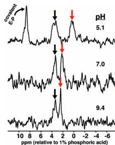
Figure 3. ^{31}\text{P} NMR of AP-bound \text{P}_i at various pH. The red arrow indicates the chemical shift of solution \text{P}_i , which is pH dependent. The black arrow indicates the pH-independent chemical shift of \text{P}_i noncovalently bound to AP. The downfield signal in the pH 5.1 sample reflects the covalently bound E-P species. The pH 5.1 sample contained 100 mM NaAcetate, 100 mM NaCl, 100 \mu\text{M} \text{ZnCl}_2 , 1 mM \text{MgCl}_2 , 2.3 mM AP, and 3.9 mM \text{P}_i . The pH 7.0 sample contained 100 mM Tris-HCl, 100 mM NaCl, 100 \mu\text{M} \text{ZnCl}_2 , 1 mM \text{MgCl}_2 , 1.1 mM AP, and 1.4 mM \text{P}_i . The pH 9.4 sample contained 100 mM NaCHES, 100 mM NaCl, 100 \mu\text{M} \text{ZnCl}_2 , 1 mM \text{MgCl}_2 , 1.8 mM AP, and 1.3 mM \text{P}_i . Stoichiometric binding of \text{P}_i is not observed at pH 9.4 as would be expected based on the relative concentrations of AP and \text{P}_i in the sample and the observed K_d value for \text{P}_i at this pH. Less than stoichiometric binding of \text{P}_i at millimolar AP concentrations has been observed previously (see refs 36 and 71 or example). An explanation consistent with the observed \text{P}_i binding at both low and high concentrations of AP is that there is only partial metal ion occupancy when AP concentrations approach or exceed the available metal ion concentrations in solution, resulting in a partial loss of \text{P}_i binding, and that this problem is exacerbated at a high pH.
